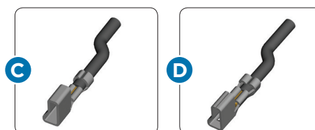
Shows a contact crimped onto a stripped wire to be inserted into a crimp housing.
