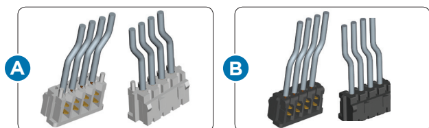
Shows unstripped wires inserted into an MT housing.
