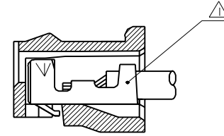
SECT. G-G
