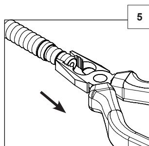
Remove outer conductor and foam.
