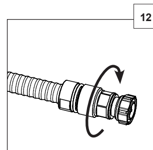
Screw the connector head onto the back nut until the thread only just grips.
