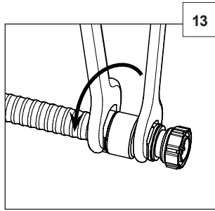
Tighten the back nut. Rotate only the back nut. Torque: 25 Nm (± 18.5 ft.-lb.)
