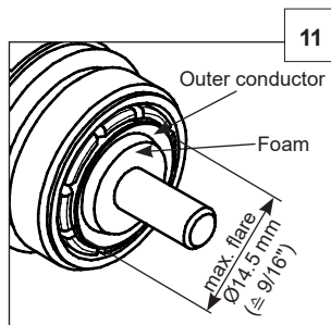
Verify the flare dimensions. Ensure the foam is fully separated and evenly spread from the cable outer conductor.
