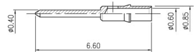
4.PIN
