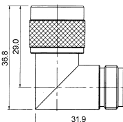
DOUBLE N FEMALE CHASSIS MOUNT
