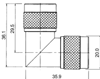
N MALE TO TNC MALE
