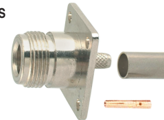
N FEMALE CHASSIS MOUNT (RG58U/59U)
