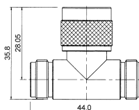
RIGHT ANGLE N MALE CLAMP TYPE (RG58U/59U/213U)
