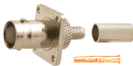
BNC FEMALE CHASSIS CRIMP TYPE (RG58U/59U)
