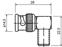
BNC MALE TO PAL FEMALE
