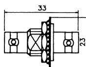
BNC FEMALE BULKHEAD CRIMP TYPE (RG174U)
