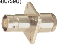
BNC FEMALE CHASSIS MOUNT CLAMP TYPE (RG58U/59U)
