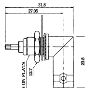
RIGHT ANGLE BNC FEMALE PANEL MOUNT
