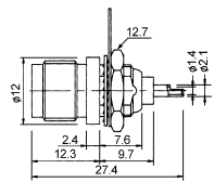
T-type triple TNC female gold-pin
