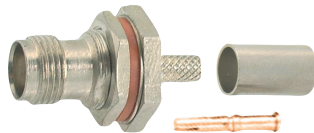
TNC female bulkhead crimp type gold-pin (RG58U/59U)
