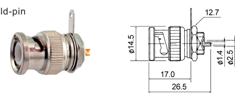
BNC female crimp type gold-pin (RG58U/59U/174U)
