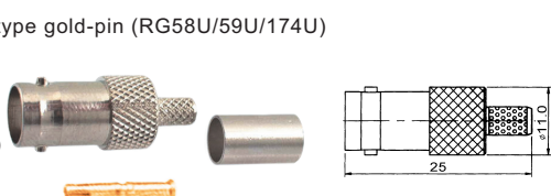
BNC female crimp type gold-pin (RG58U/59U/174U) teflon insulation
