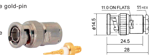
BNC male clamp type gold-pin (RG58U/59U) teflon insulation
