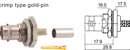
BNC female bulkhead crimp type gold-pin (RG58U/59U/174U) teflon insulation
