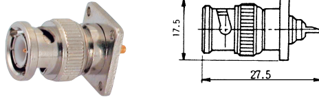
BNC male chassis mount gold-pin
