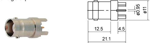
BNC female PCB mount gold-pin teflon insulation
