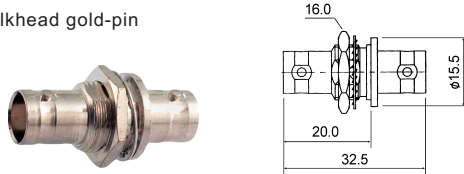
Double BNC female bulkhead gold-pin
